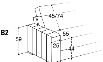
SPALLIERA SFODERABILE REMOVABLE UPHOLSTERY FOR BACK CUSHIONS COUSSINS DOSSIER DÉHOUSSABLES
